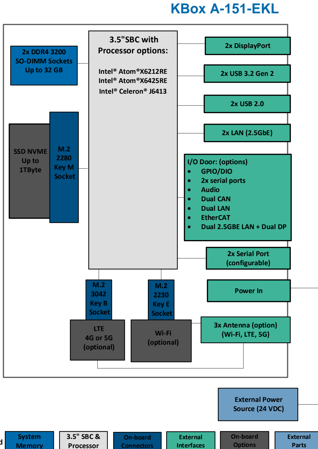
Figure 24: Block Diagram KBox A-151-EKL
