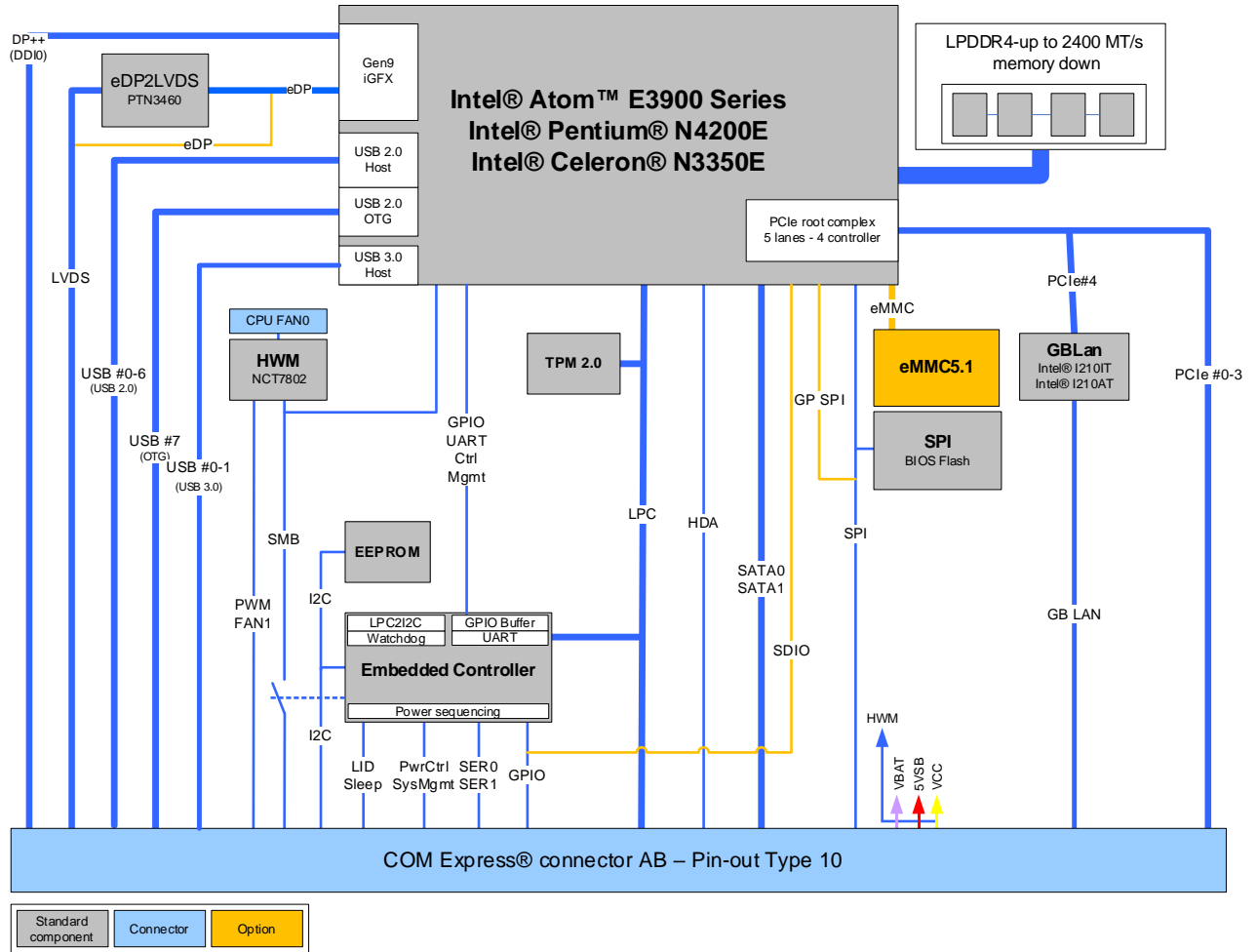
Figure 2: Block Diagram COMe-m4AL10
